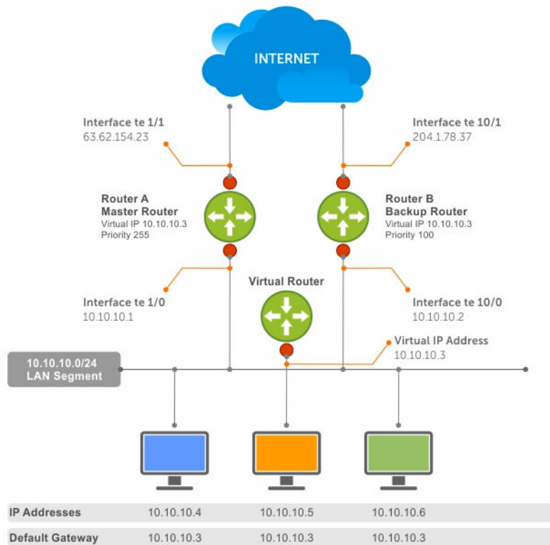
Figure 125. Basic VRRP Configuration
